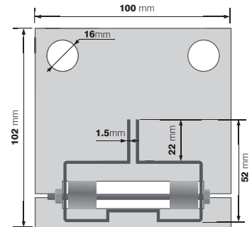
Upright M70 (with footplate) -use M12 floor fixing
