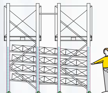
After – Dynamic storage
