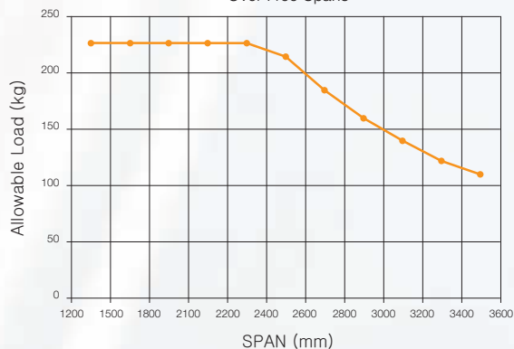
Versi Flow: Allowable Tracks Loads Over Free Spans
